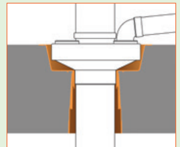
Cross-section of QuelCast Cast In Fire Collar installed with a Manifold on the Top
