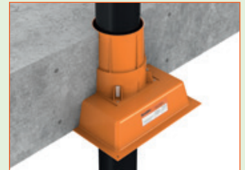
QuelCast Cast In Fire Collar installed with a Manifold on the Bottom
