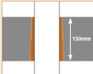
Cross-section of QuelCast Cast In Fire Collar Cut to Suit a 150mm Floor Slab
